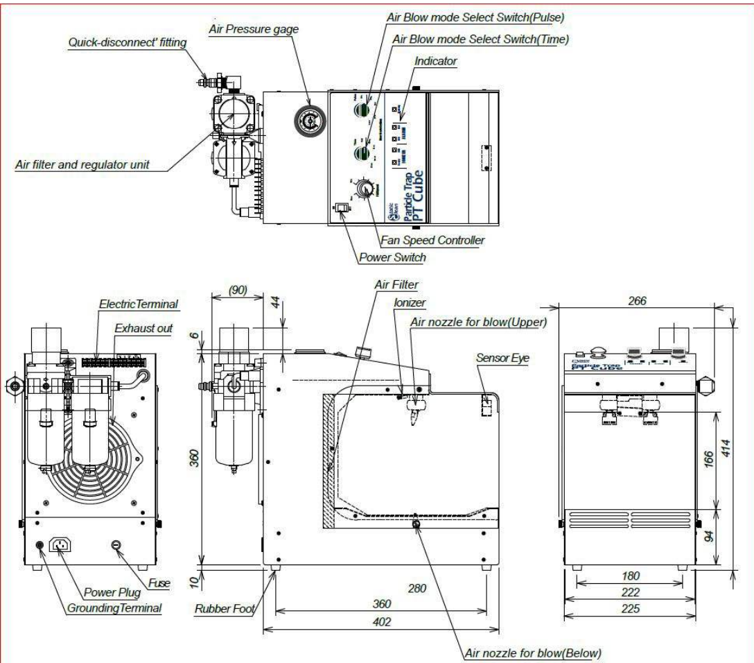
Dimensional Drawing
