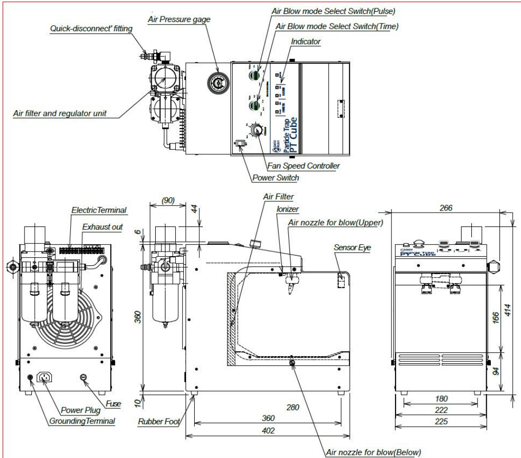
Dimensional Drawing
